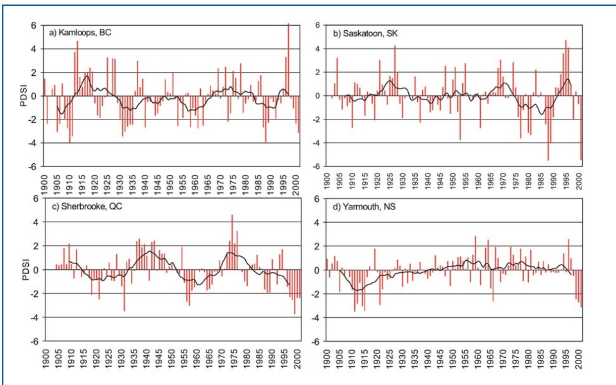
Fig. 2. Annual PDSI values for a) Kamloops, BC, b) Saskatoon, SK, c) Sherbrooke, QC, and d) Yarmouth, NS. Solid lines represent 10-year running means (source: Climate Research Branch, Meteorological Service of Canada, Environment Canada, Downsview, ON).
